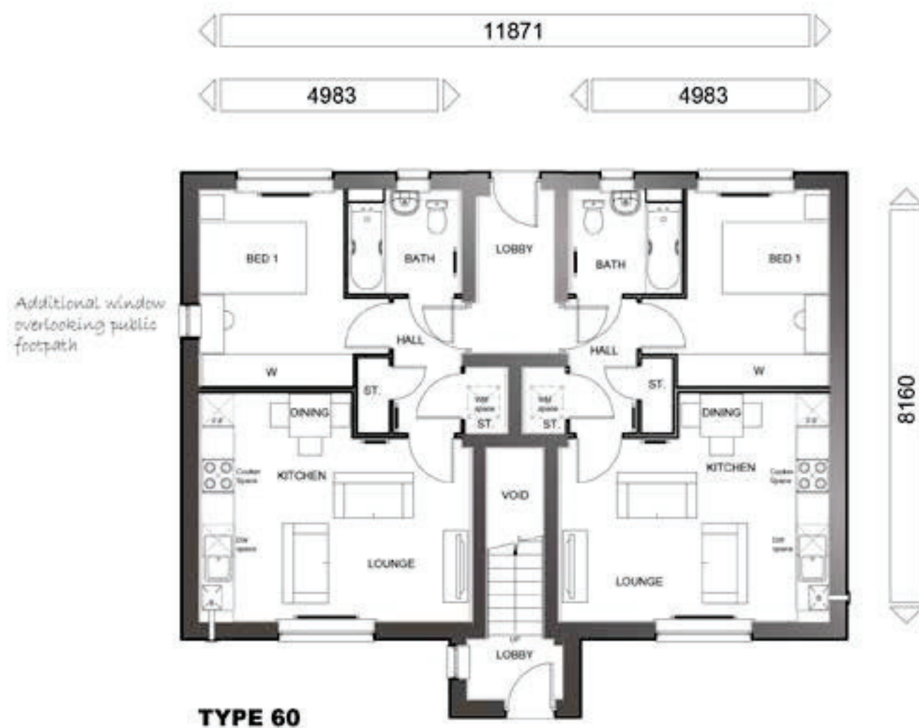
Ground Floor Plan - Type 60
