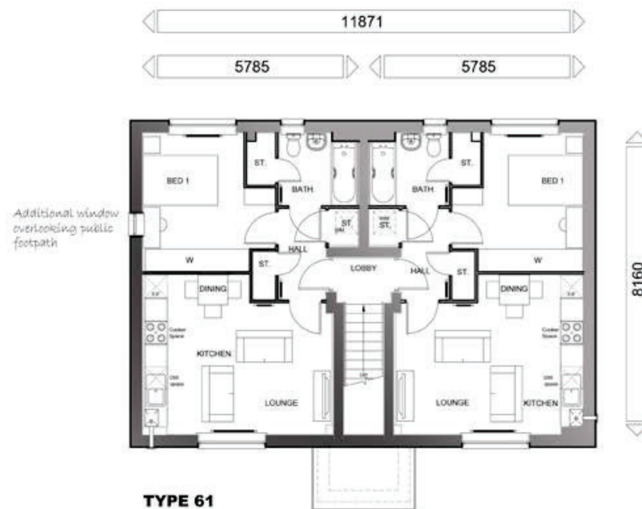
First Floor Plan - Type 61
