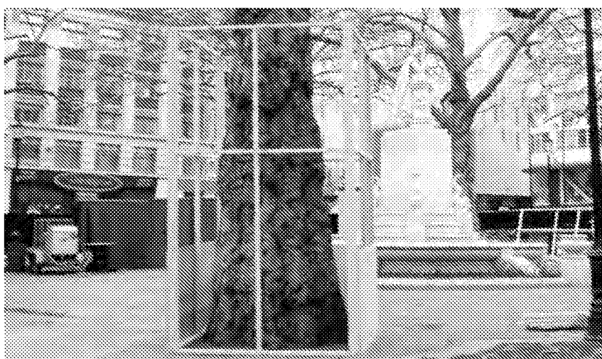
SGN 2-08 A wood frame around the trunk can be used to support a plywood surround.
