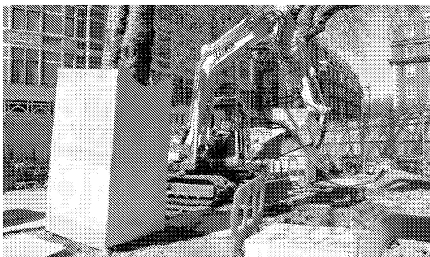
SGN 2-07 Boards attached to a supporting framework surrounding the trunk reduces the risk of accidental impact.
