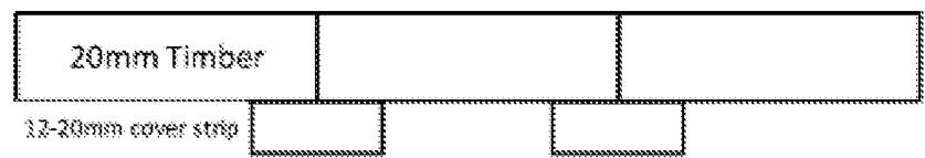
Figure 14. Using batons to cover the fencing joins on an acoustic fence
