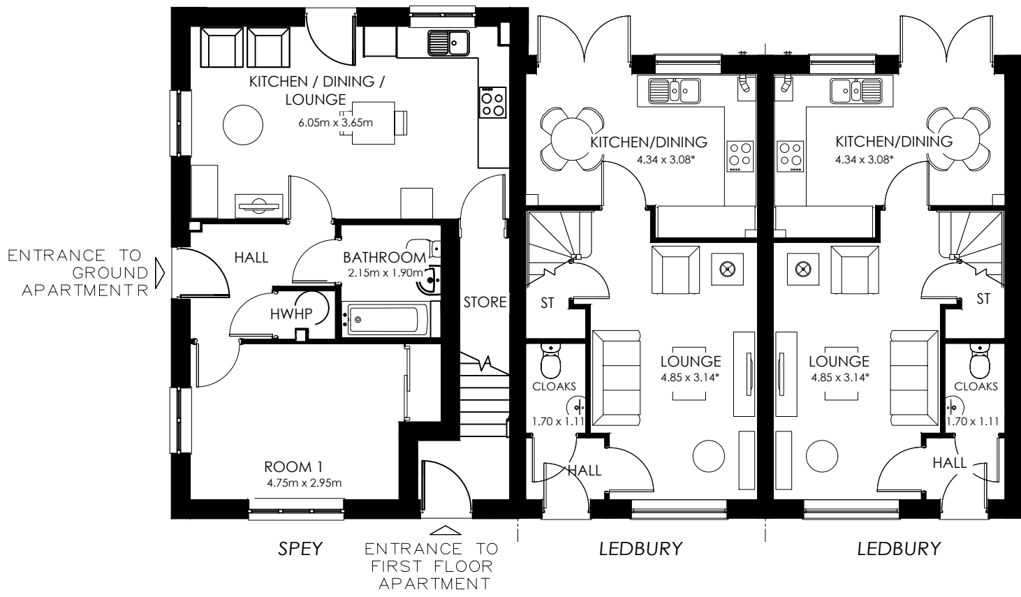
Ground Floor
