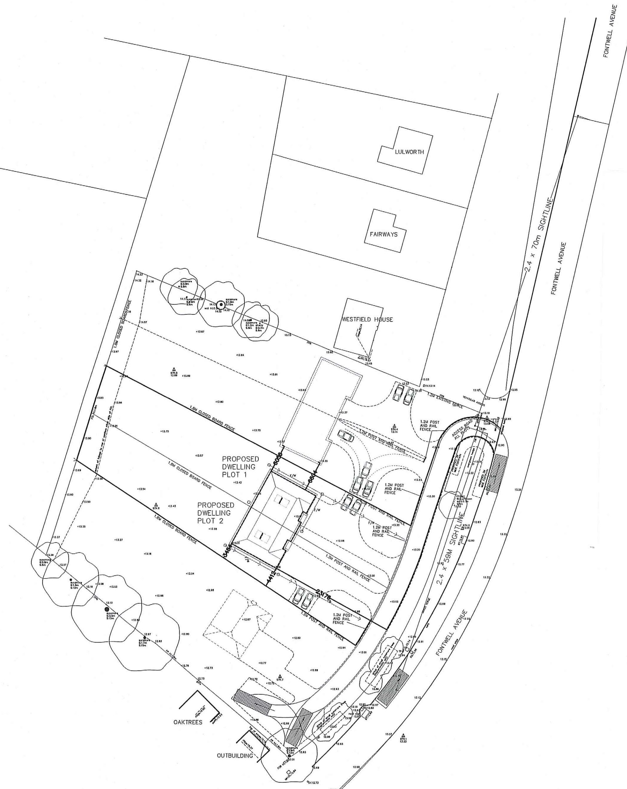
BLOCK PLAN 1:500
