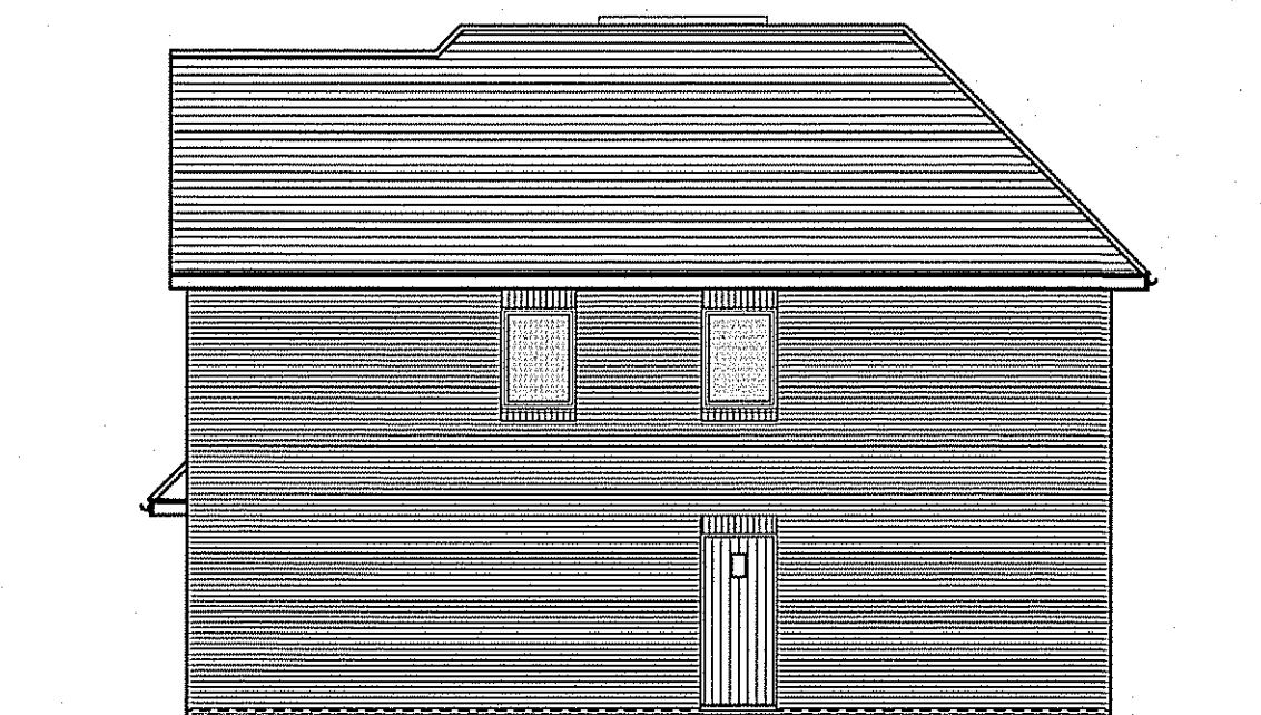
NORTH FACING ELEVATION
