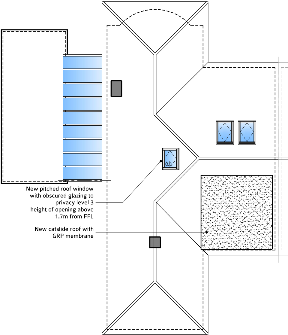
ROOF PLAN AS PROPOSED 1:100
