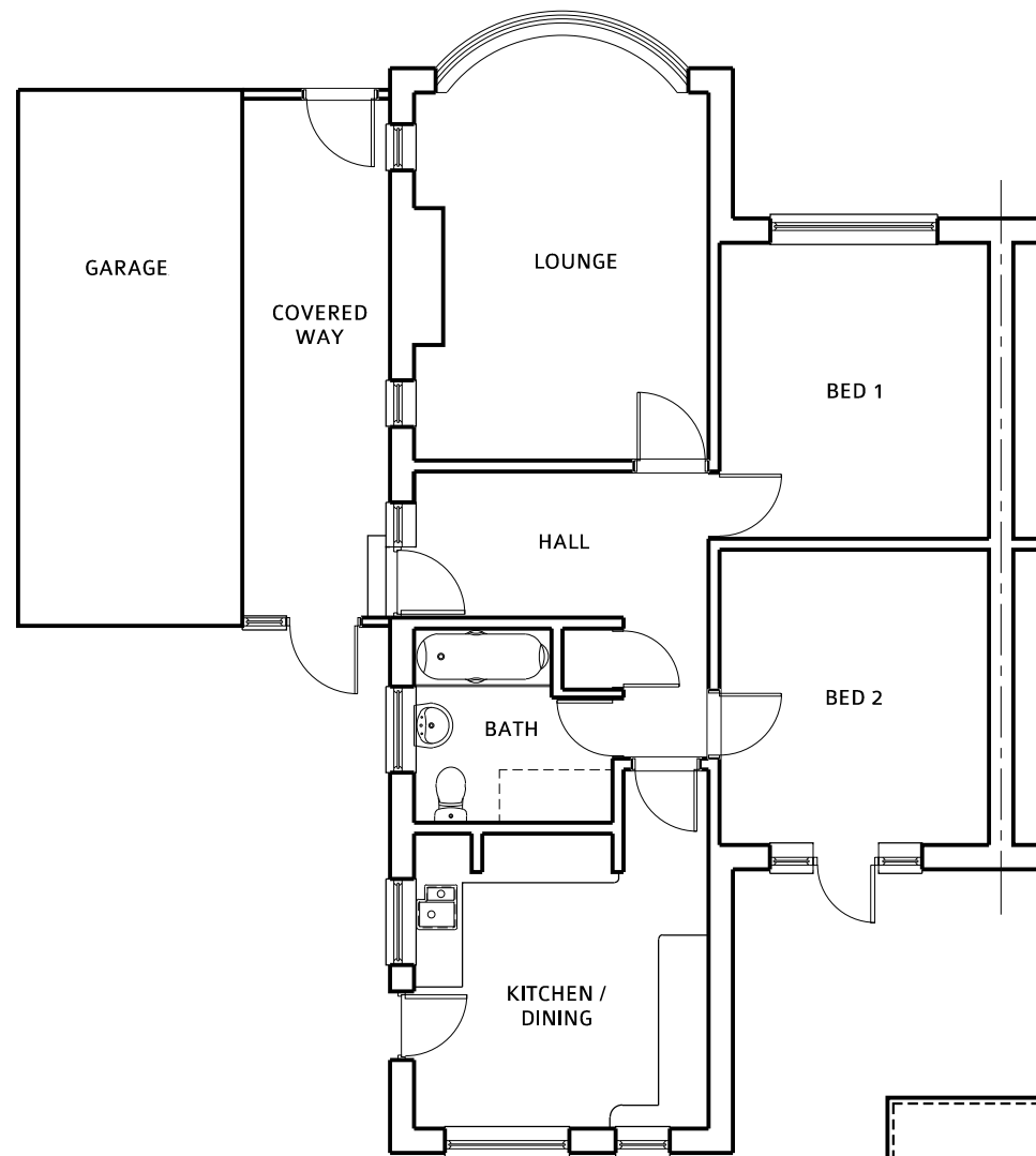
GROUND FLOOR PLAN AS EXISTING 1:100
