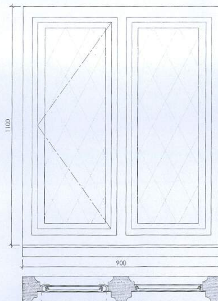
TYPE 1 AS PROPOSED (Fan lights replaced with fixed casements)
