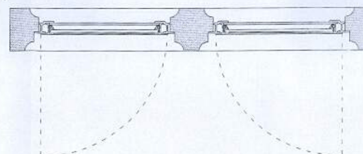
TYPE 2 AS PROPOSED (Side hung casements to match the existing)
