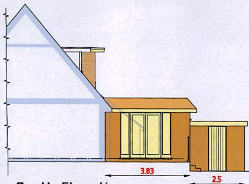
South Elevation Including Store
