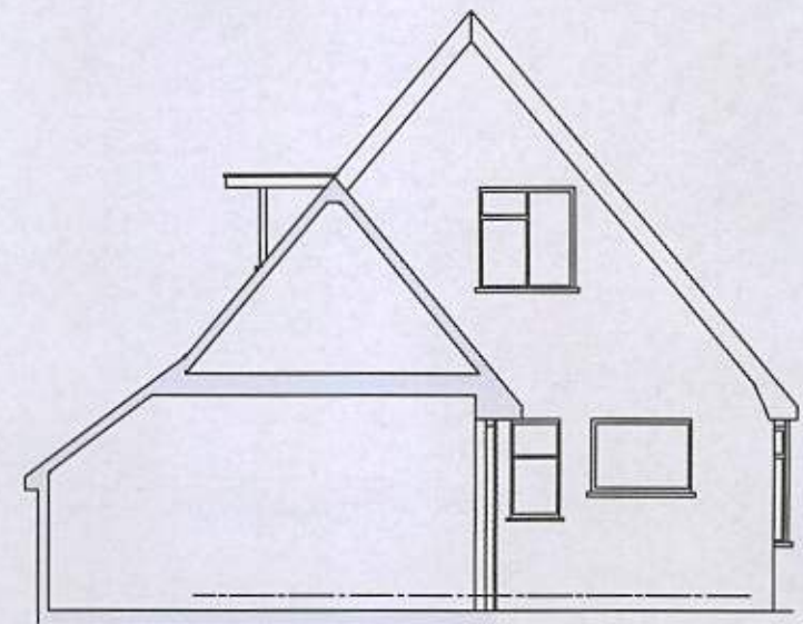
North Elevation
