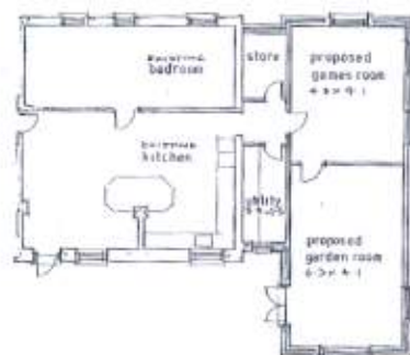
PART GROUND FLOOR PLAN 1:100
