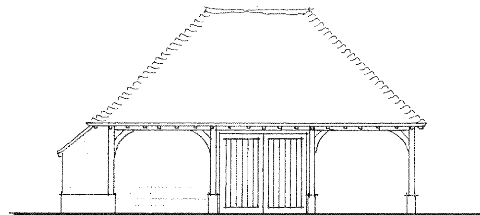
West Elevation
