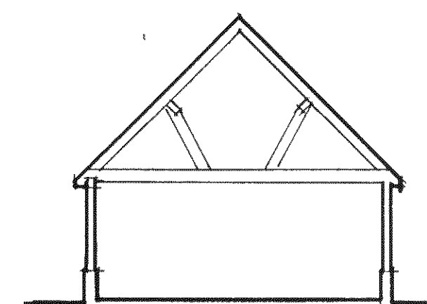
Cross Section
