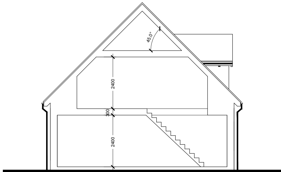
Typical Section
