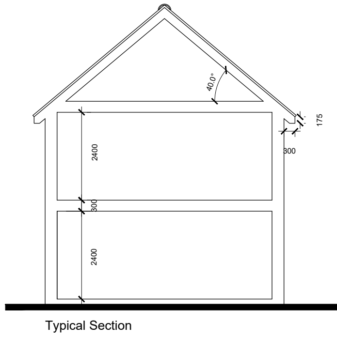
Typical Section
