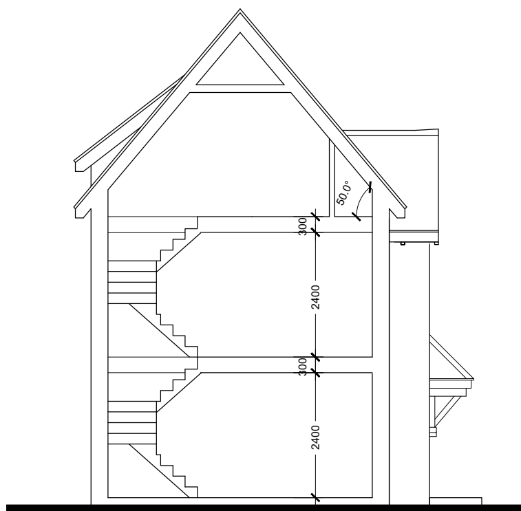
Typical Section
