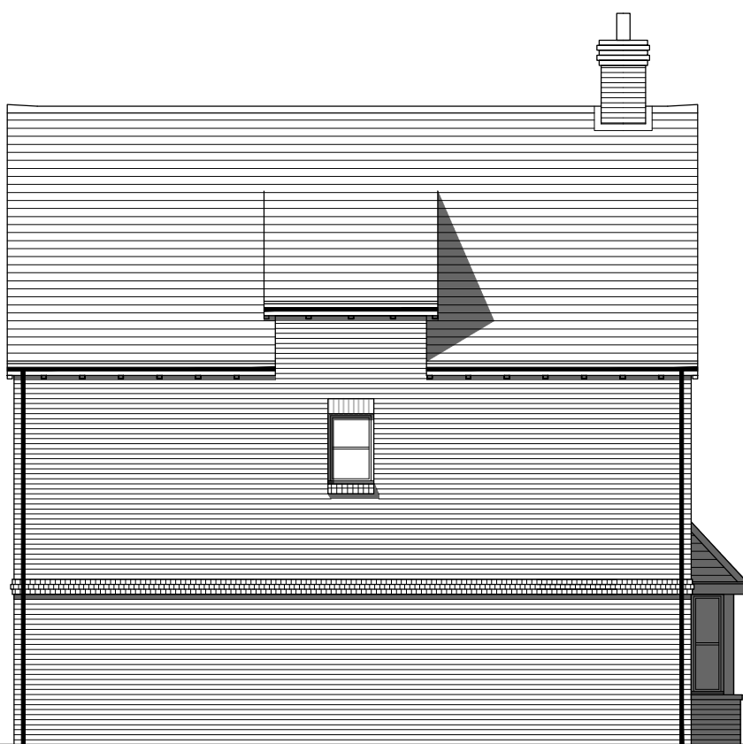
Rear Elevation Plots as drawn 72, 88 Plots handed 26, 73, 89, 101
