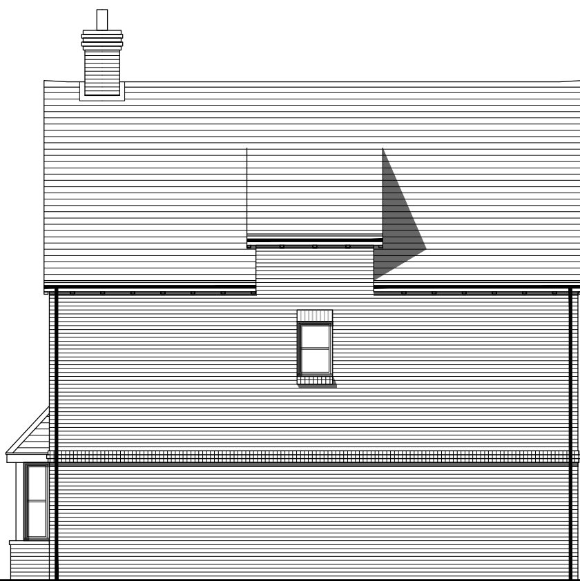
Rear Elevation
