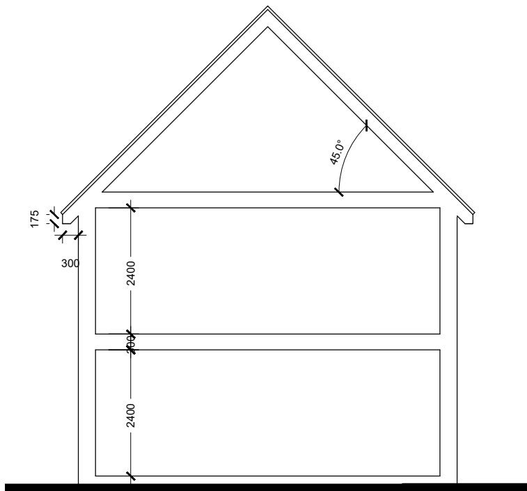
Typical Section
