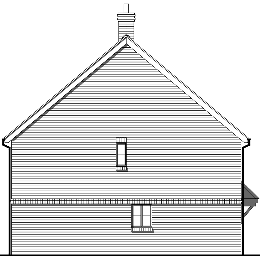
Side Elevation
