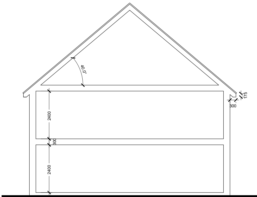
Typical Section
