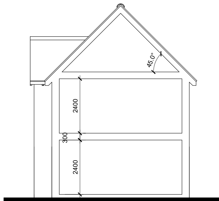
Typical Section
