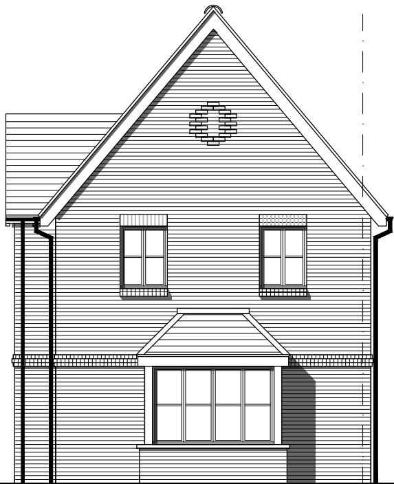
Side Elevation
