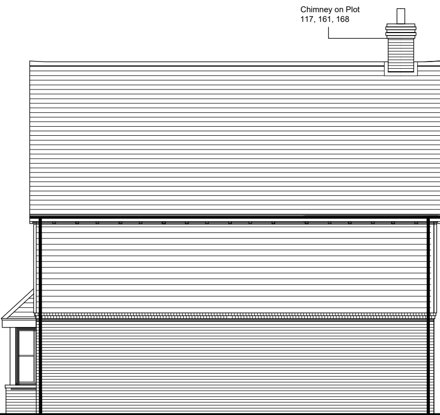
Rear Elevation
