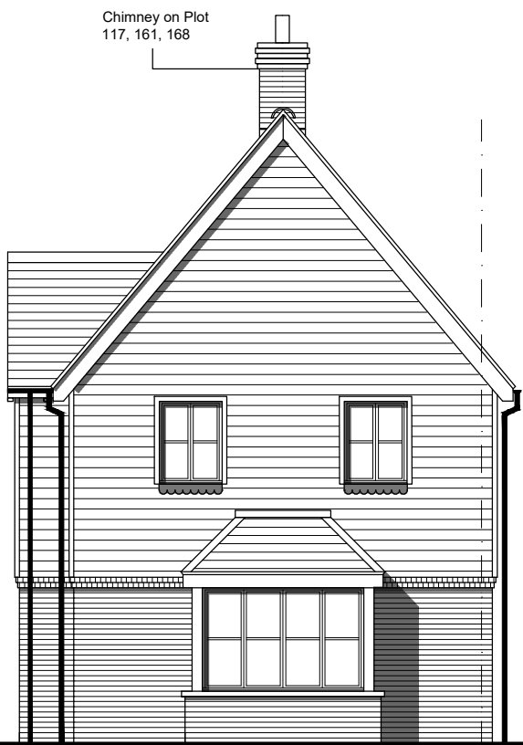
Side Elevation
