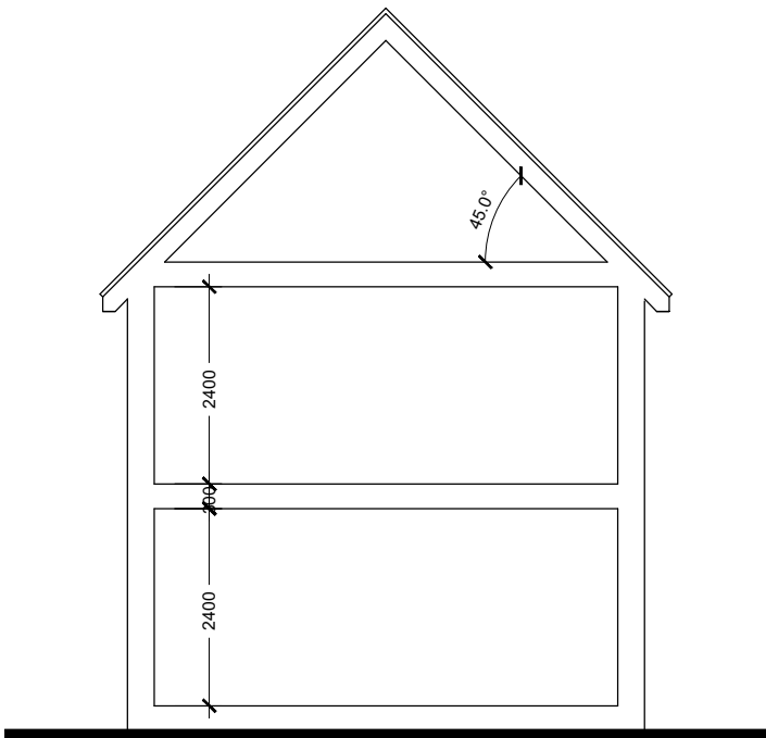
Typical Section
