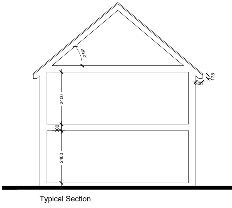
Typical Section
