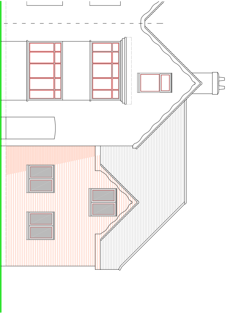
FRONT ELEVATION
