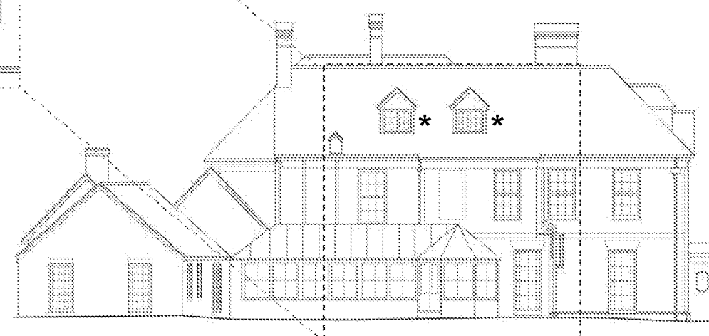
West Elevation
