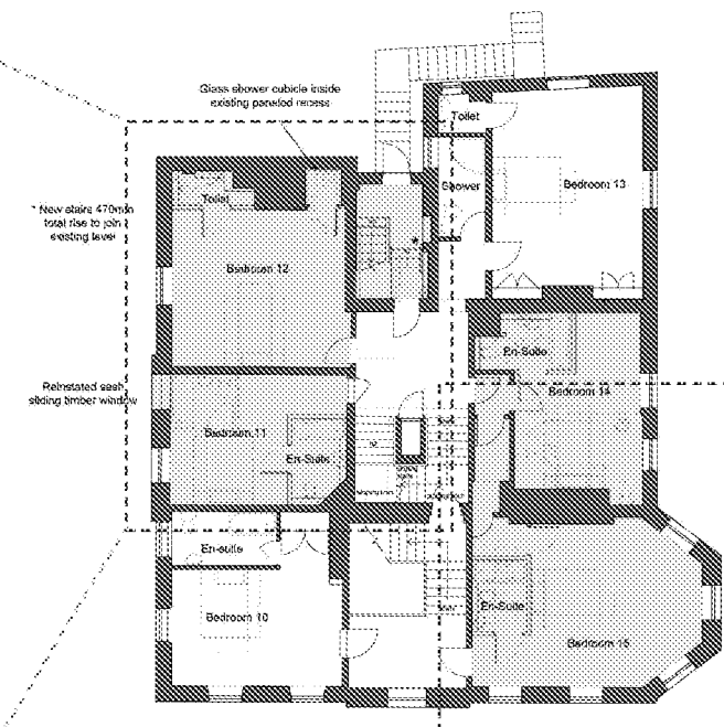
Fig : Existing First Floor Plan
