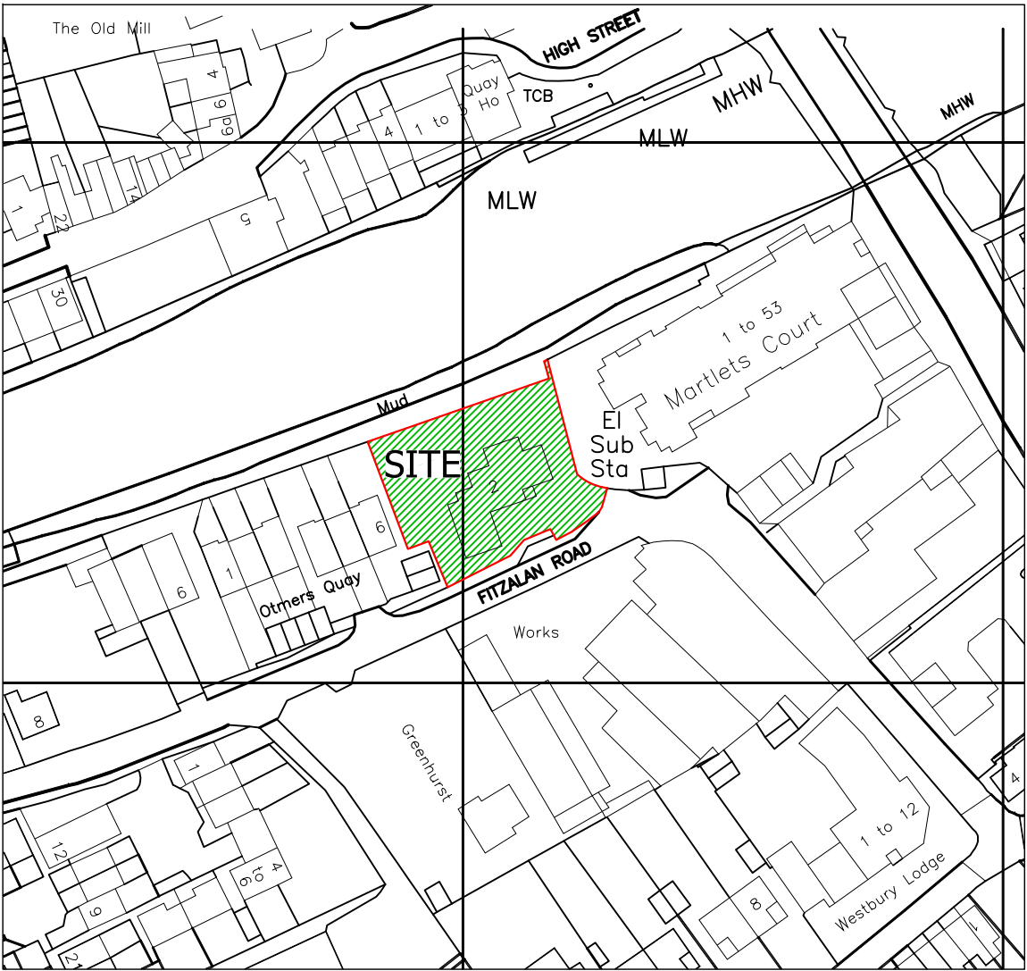
EXISTING LOCATION PLAN, Sc. 1:1250
