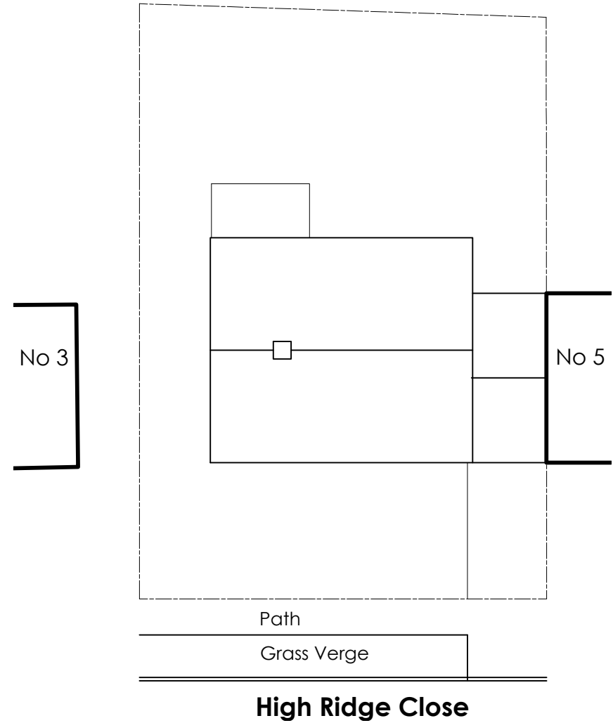
Block & Site plan 1:200 @ A3
