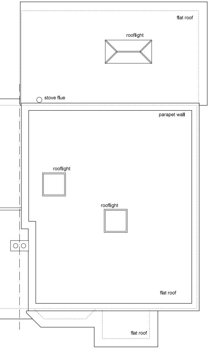
Roof Plan
