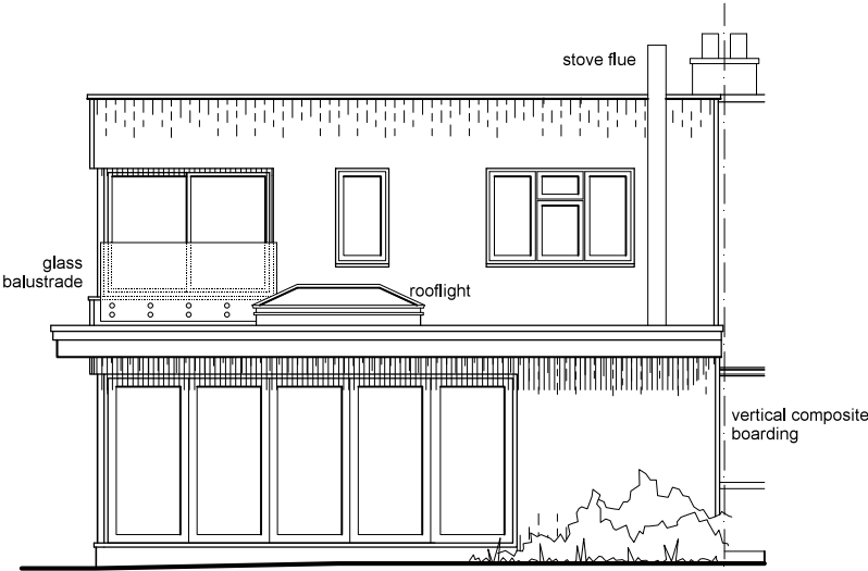
South East Elevation
