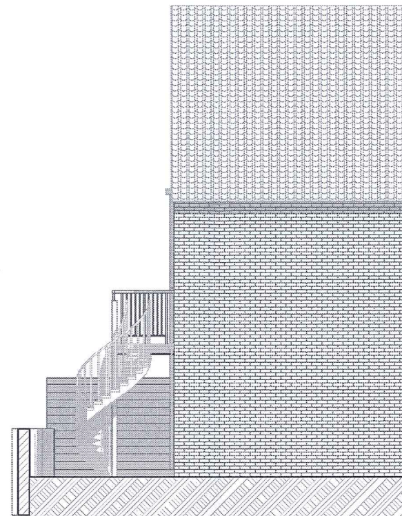
East Elevation
