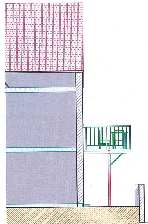
West Elevation
