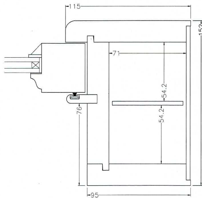
PLAN SECTION
