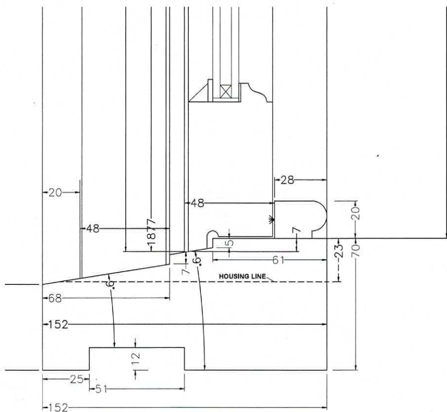
HEIGHT SECTION
