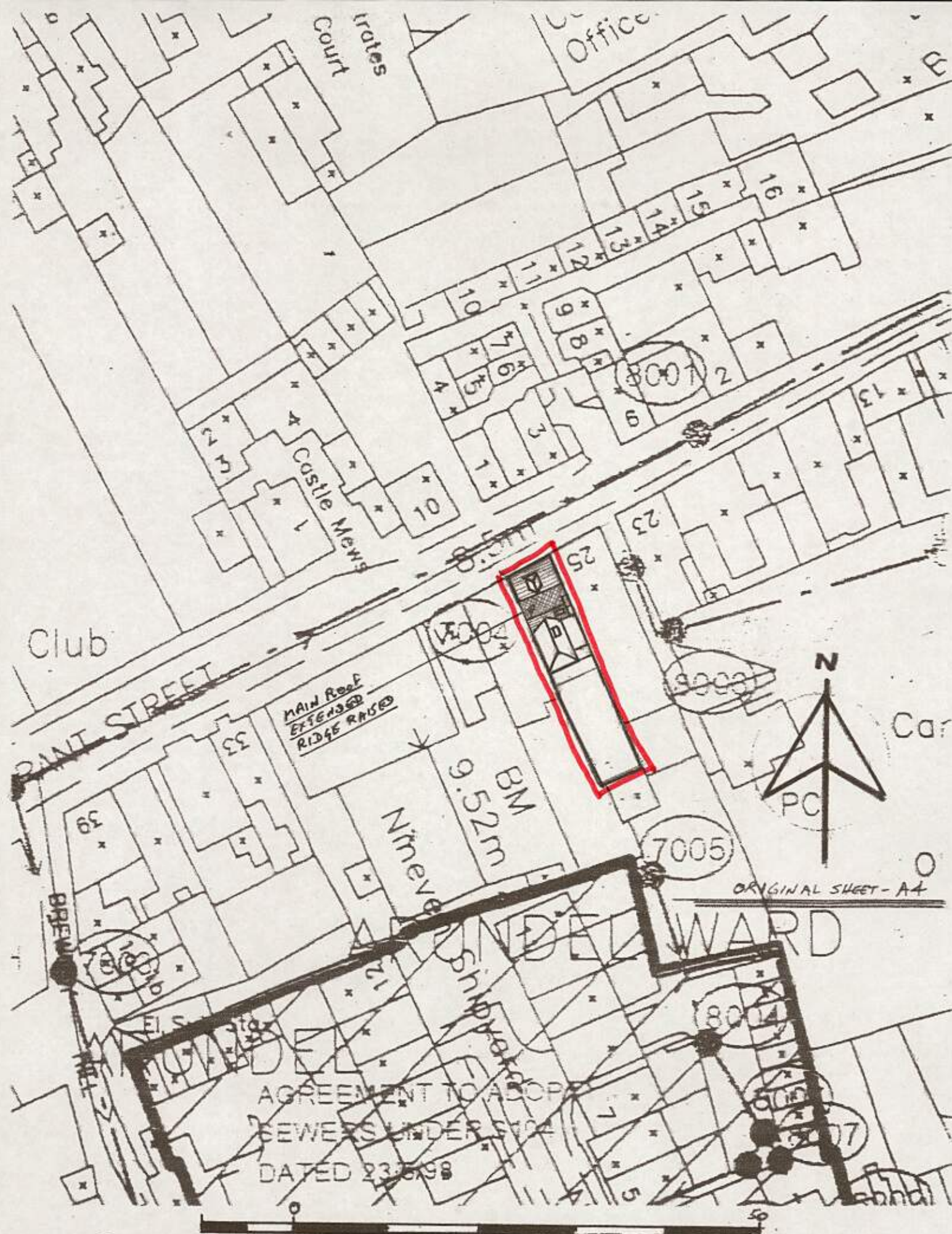
27A TARRANT STREET, ARUNDEL. BLOCK PLAN 1:500
