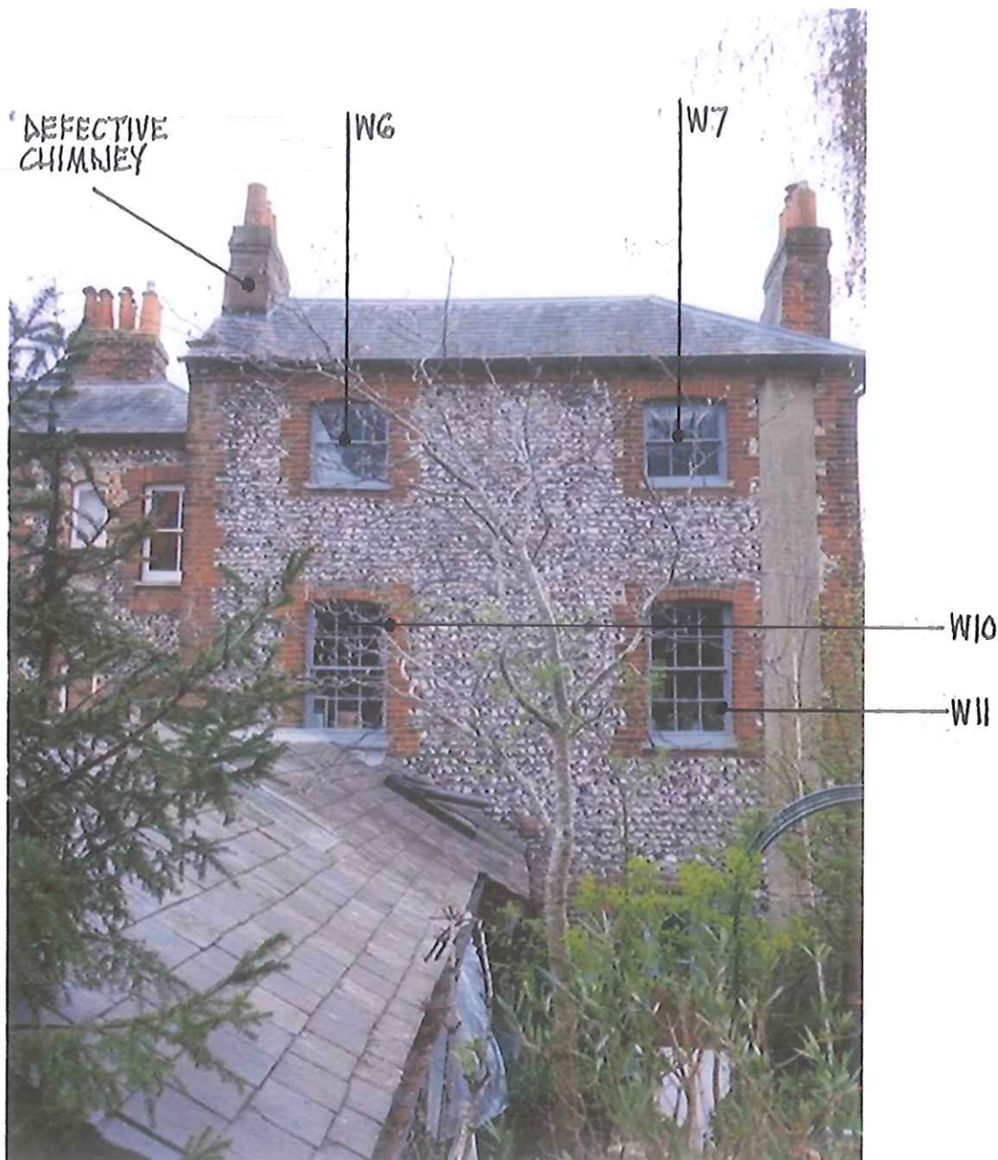
REAR ELEVATION - CHIMNEY AND WINDOWS 6, 7, 10 + 11
