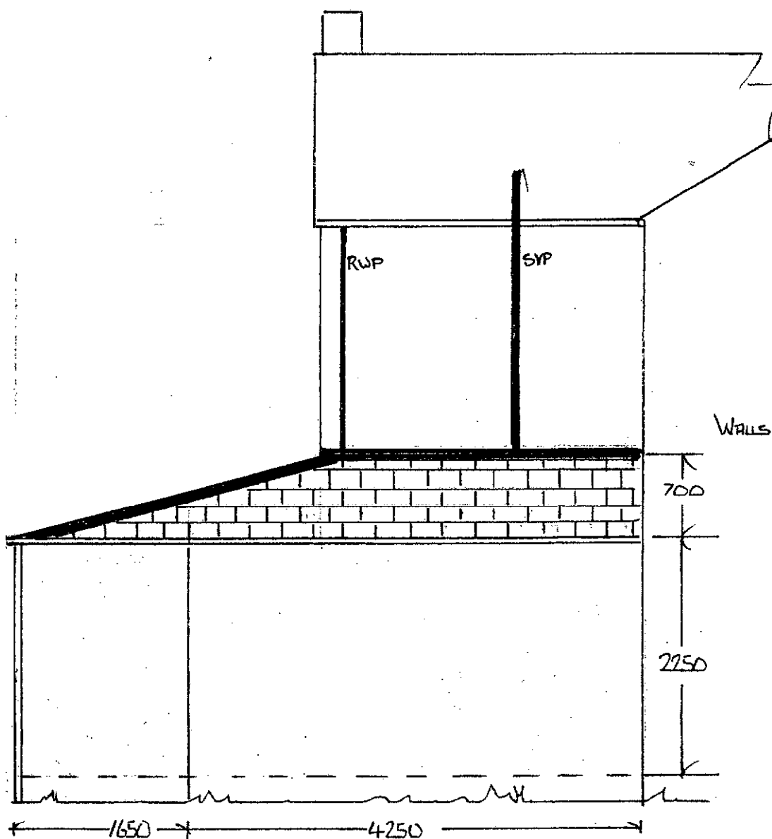
PROPOSED NEW SIDE ELEVATION
