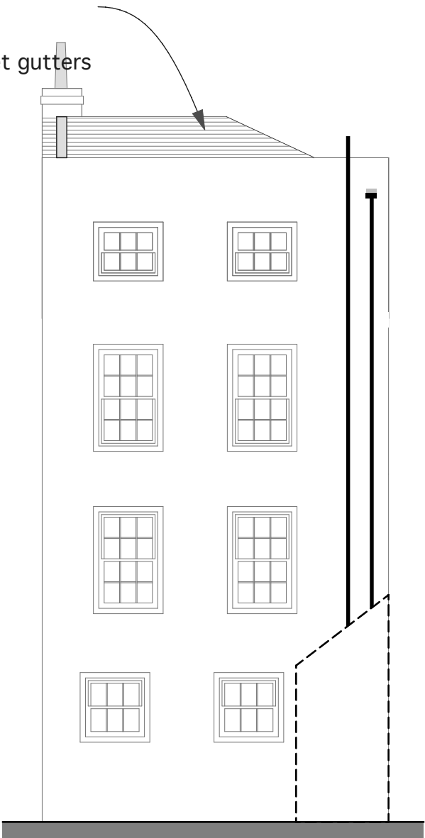
Rear South Elevation - proposed
