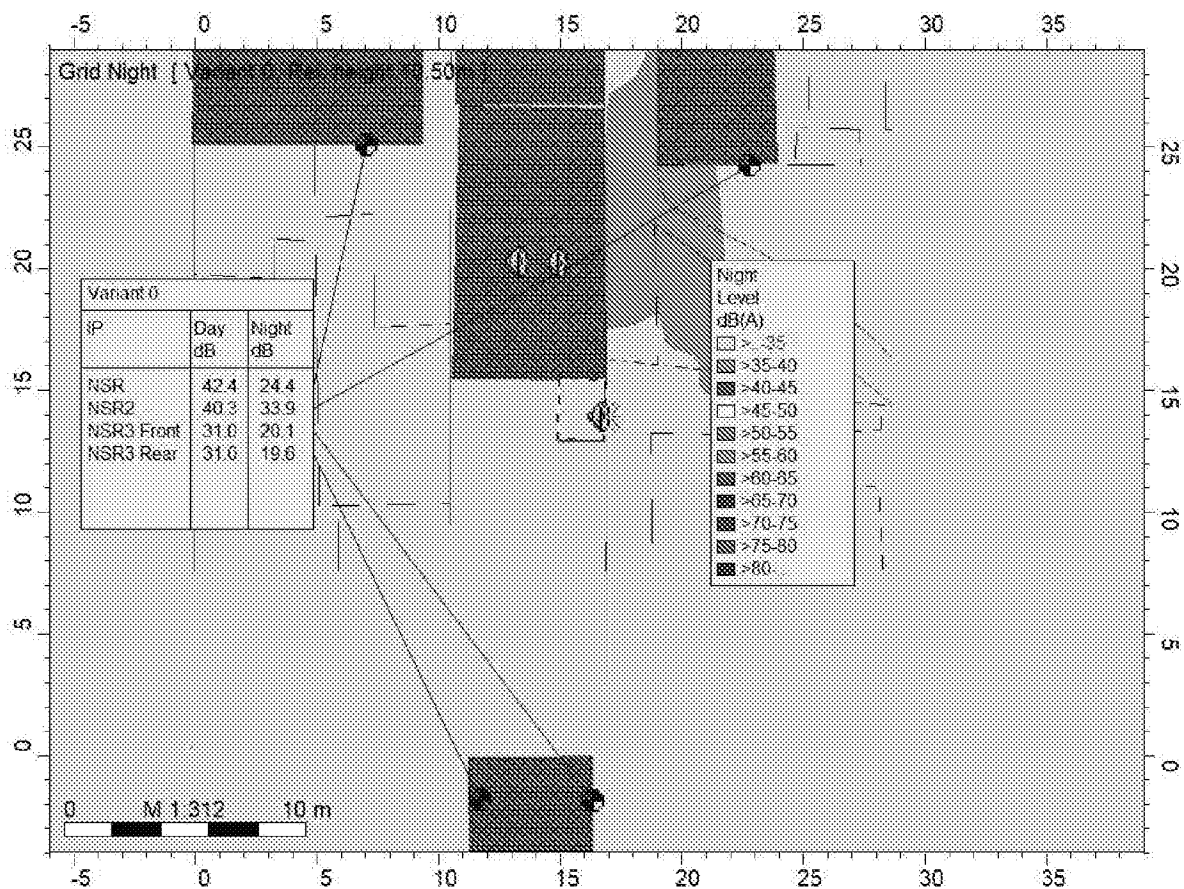
Figure 6: Night Time Noise Model
