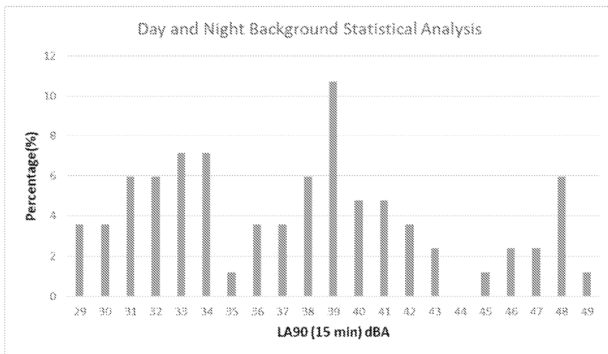
Figure 4: 11:00-07:00hrs L90 Analysis
