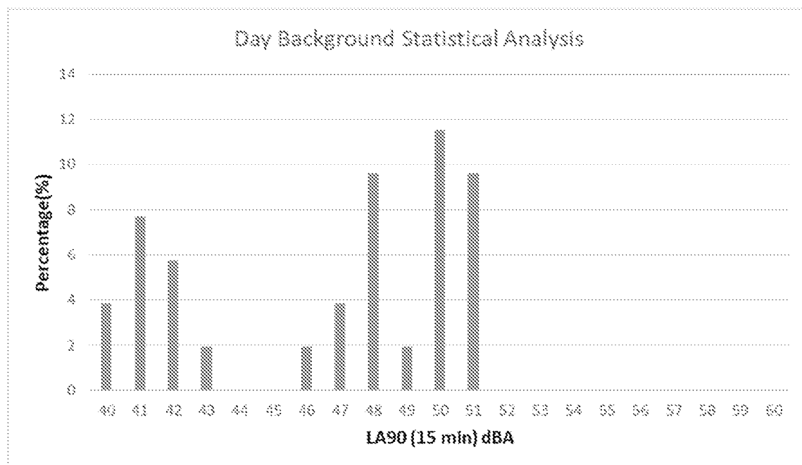
Figure 3: 11:00-23:00 L90 Analysis
