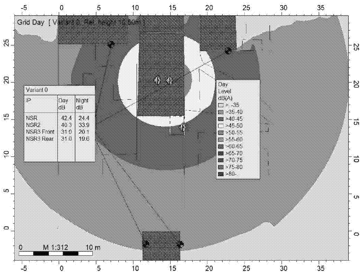
Figure 5: With Mitigation Day Noise Model
