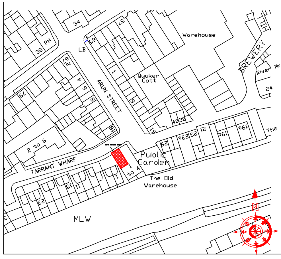
Location Plan 1 : 1250
