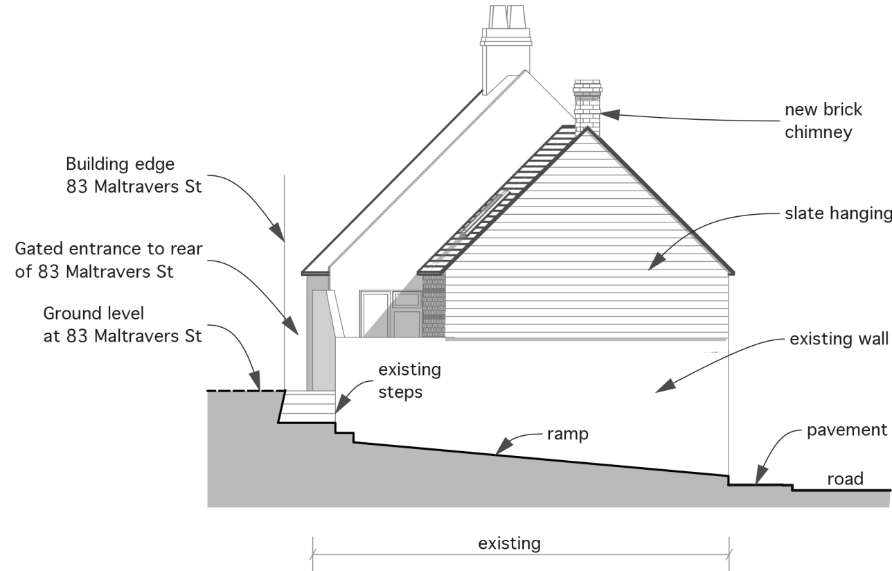
North Elevation proposed
