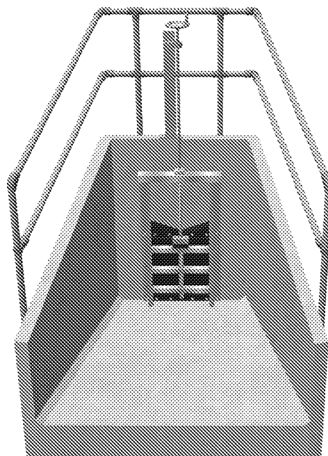
Penstock
