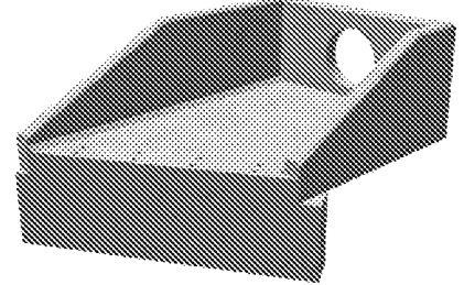
R18A 05 3210 LH 1:2 Wing Wall 2 Piece Headwall
