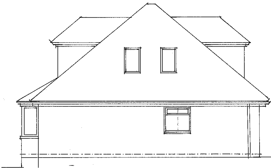
NORTH ELEVATION
