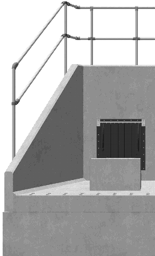
Stepped Baffle Blocks
