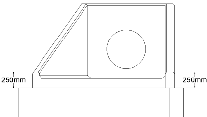
AH12C Right Hand Angled Headwall
