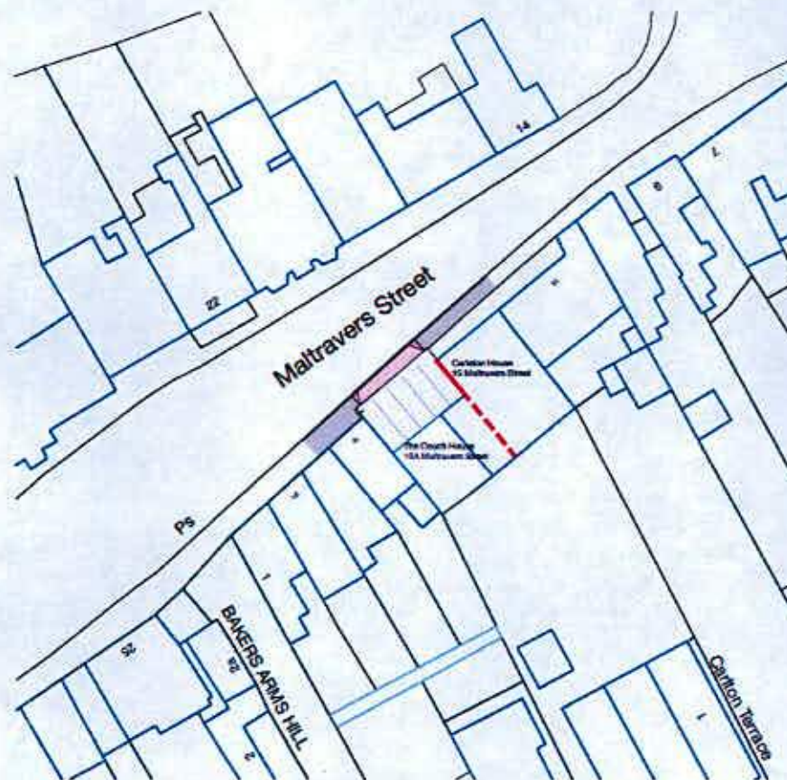
Block Plan 1:500
