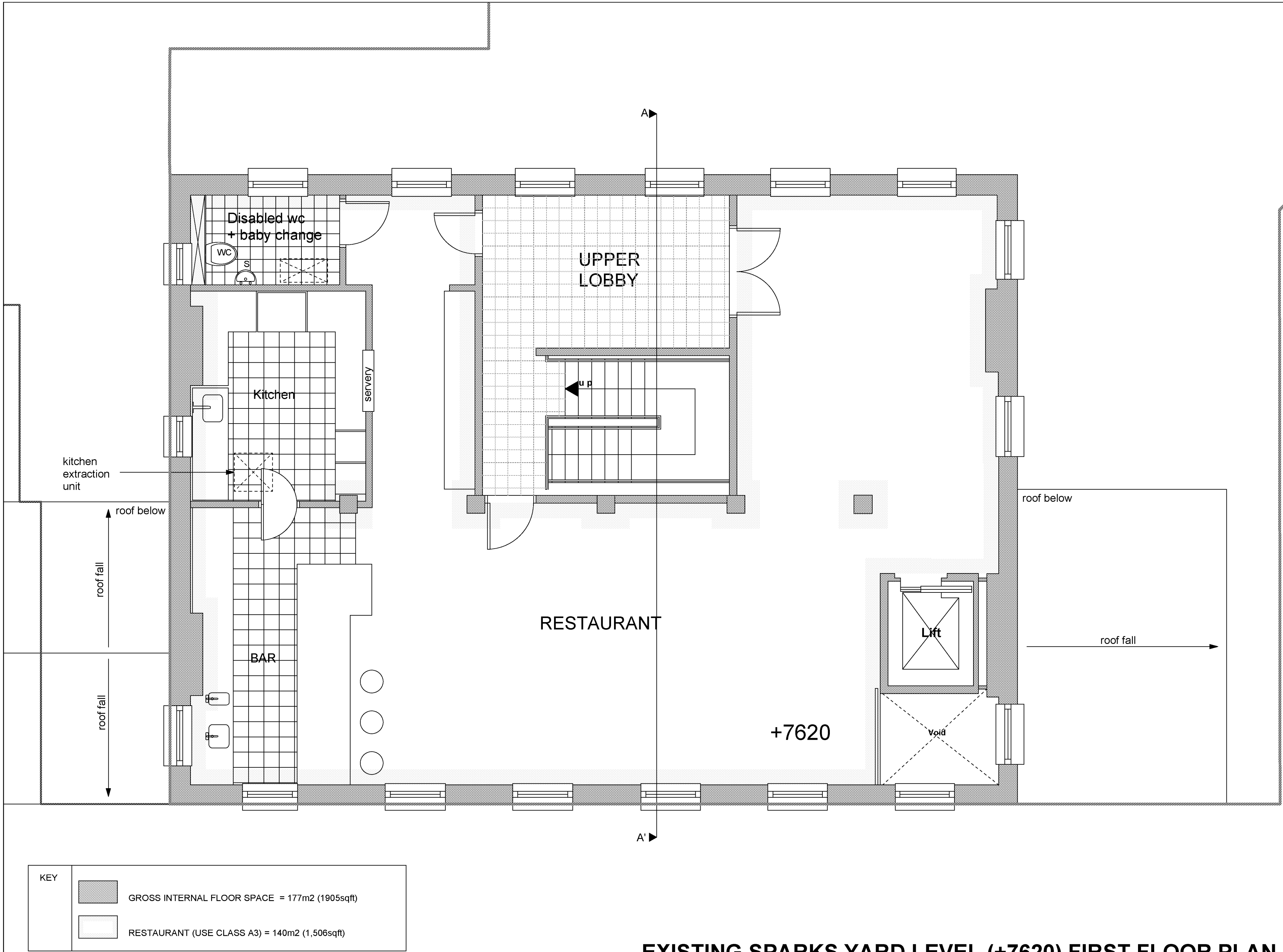
EXISTING SPARKS YARD LEVEL (+7620) FIRST FLOOR PLAN
