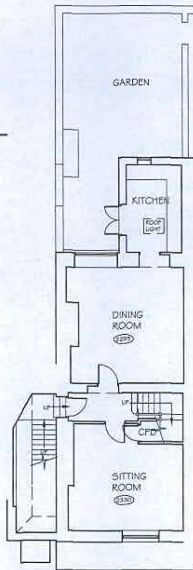
EXISTING FIRST FLOOR
