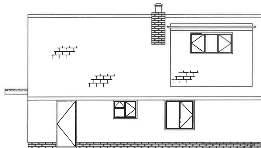
North West Section X-X
