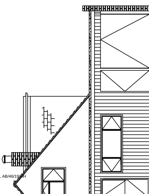
on 'A' (North East - Front Elevation)
