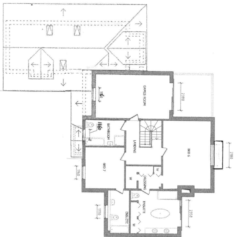
PROPOSED THIRD FLOOR PLAN
