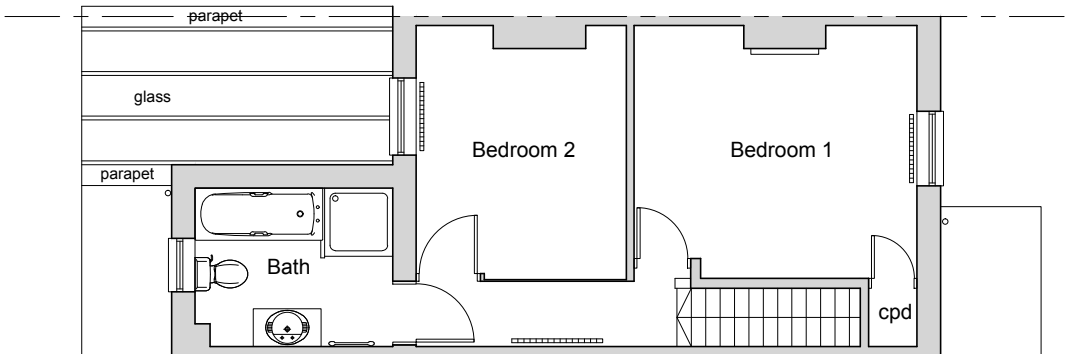
Pr. First floor plan 1:100 @ A3
