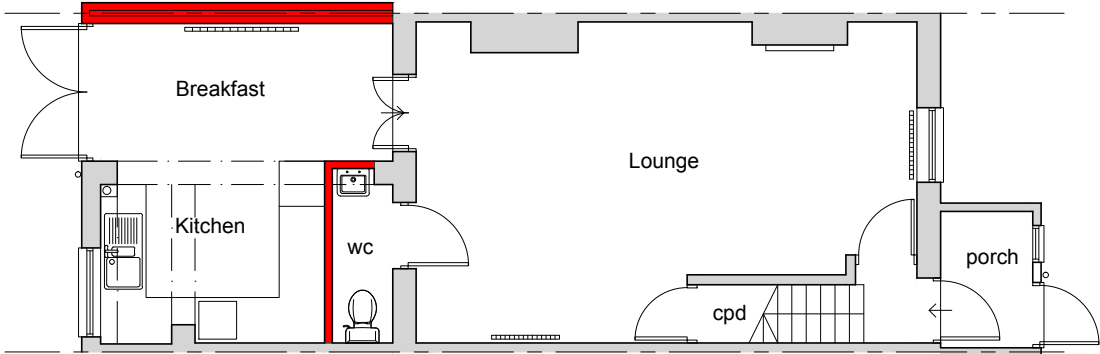
Pr. Ground floor plan 1:100 @ A3
