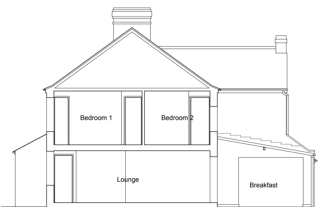
Pr. North Elevation (section) 1:100 @ A3
