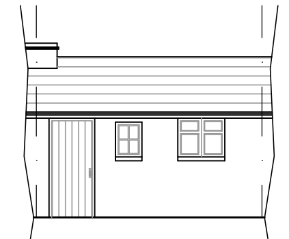
South Elevation (Outhouse)
