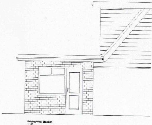
Existing West Elevation 1:100
