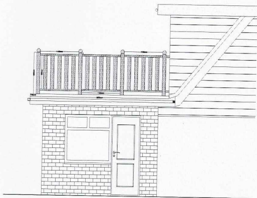
Proposed West Elevation 1:100
