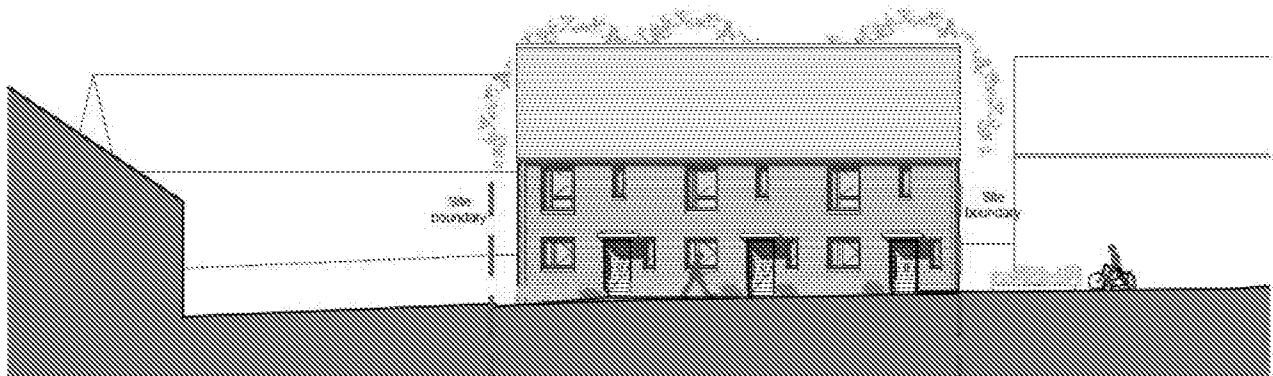
Figure : Proposed site section
